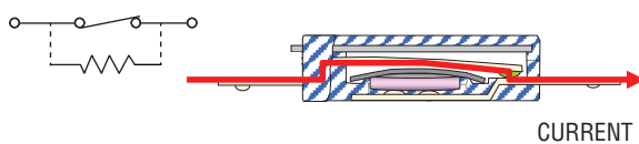
NORMAL CIRCUIT
