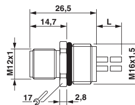
Dimensional drawing
