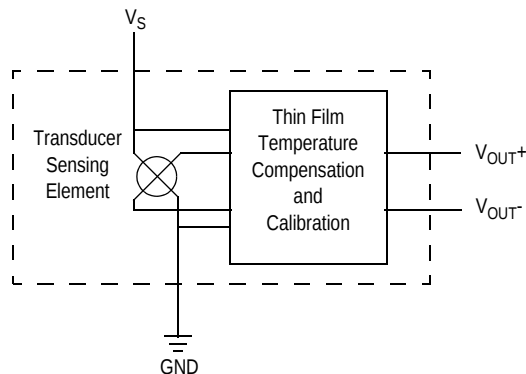
Figure 1. Integrated pressure sensor block diagram
