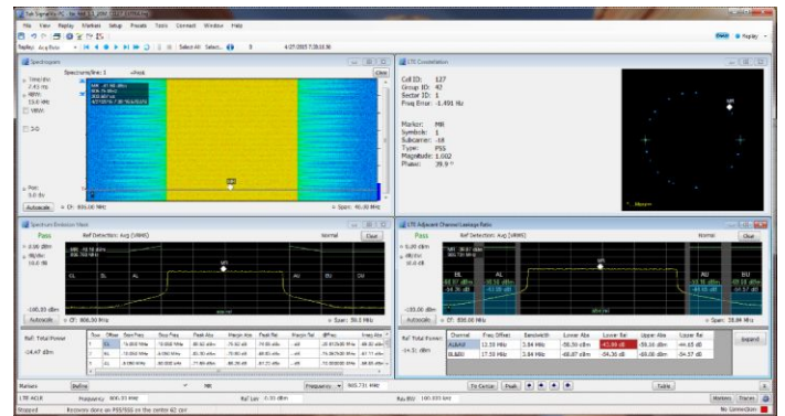
Fast validation of LTE base station transmitter with push button preset, and pass/fail information
