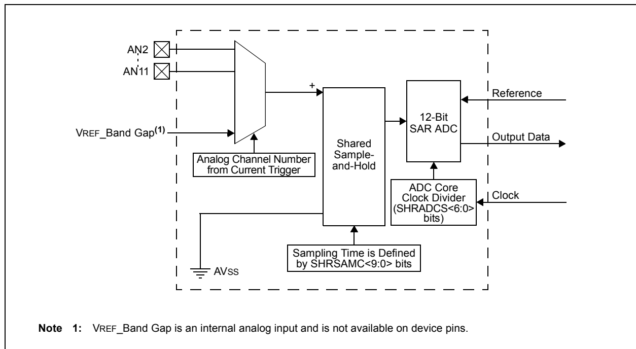
FIGURE 19-3: SHARED CORE BLOCK DIAGRAM
