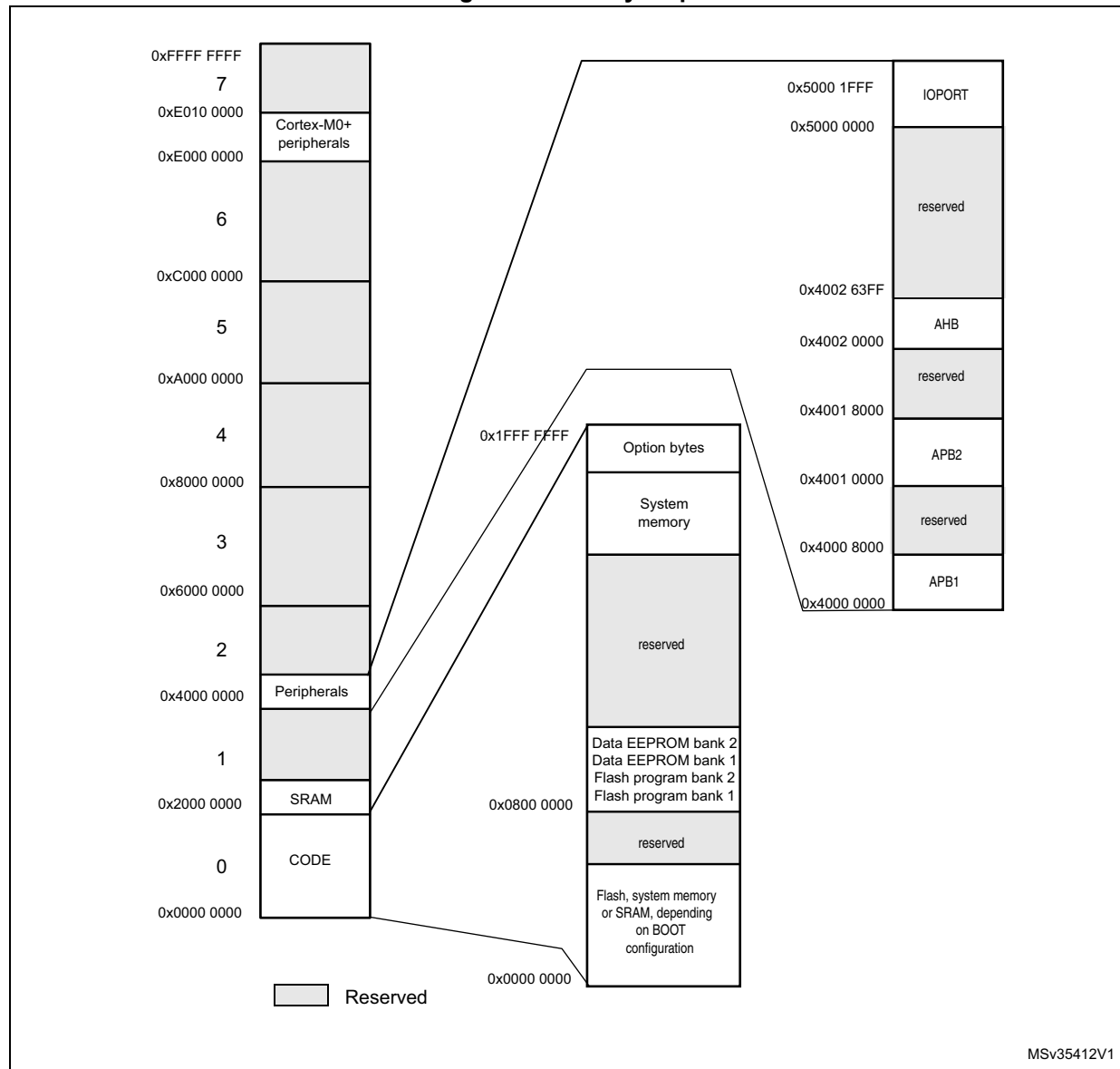
Figure 8. Memory map
