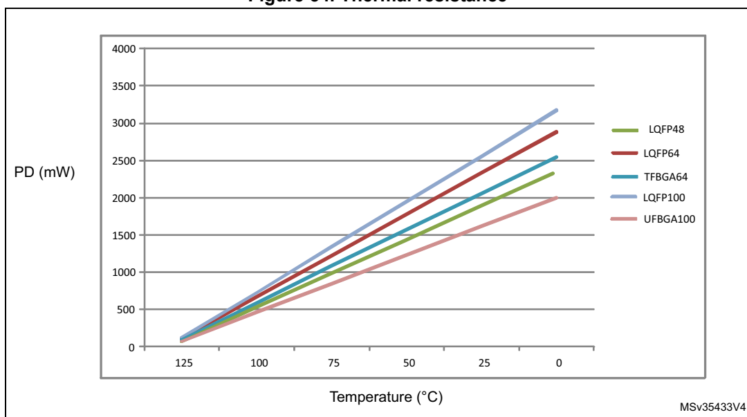
Figure 54. Thermal resistance
