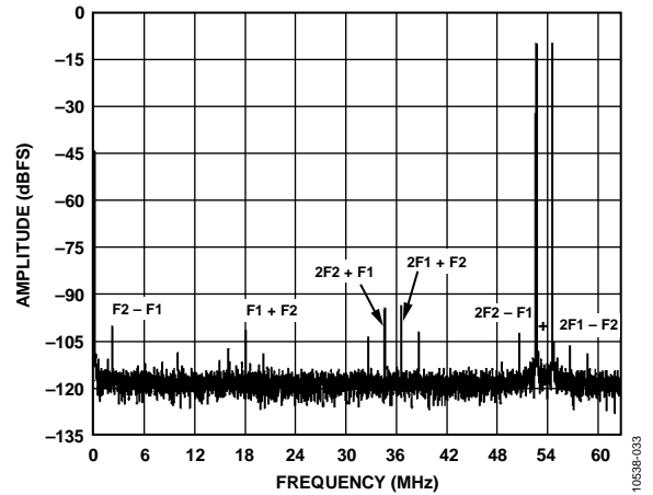
Figure 33. Two-Tone 16k FFT with f_{IN1} = 70.5 MHz and f_{IN2} = 72.5 MHz, f_{SAMPLE} = 125 MSPS, V_{REF} = 1.3 V
