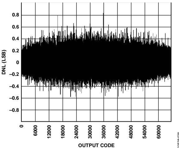
Figure 38. DNL, f_{IN} = 9.7 MHz, f_{SAMPLE} = 125 MSPS, V_{REF} = 1.3 V
