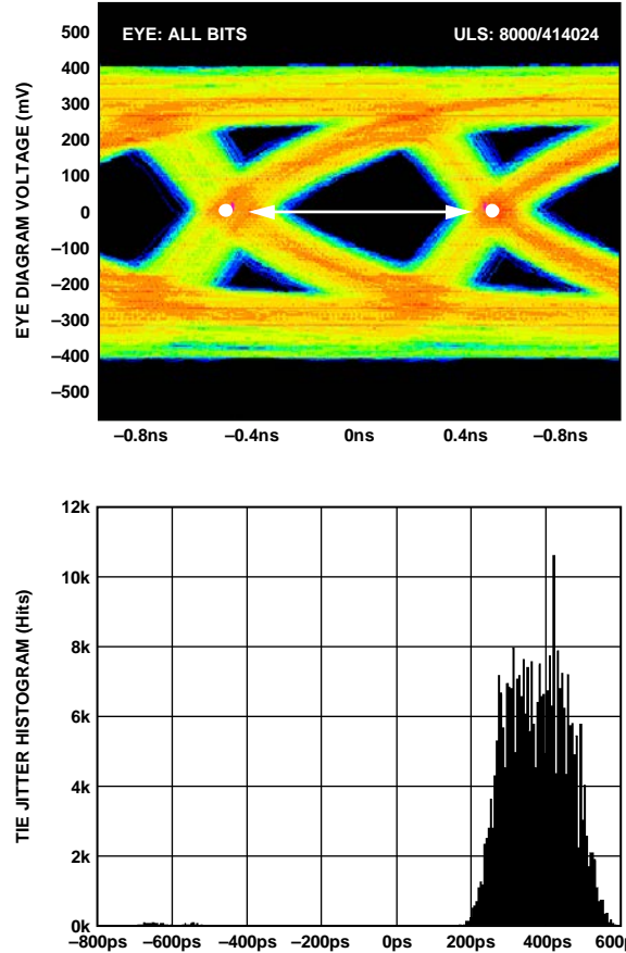
Figure 74. Data Eye for LVDS Outputs in ANSI-644 Mode with Trace Lengths Greater than 24 Inches on Standard FR-4 Material, External 100 Ω Far-End Termination Only
