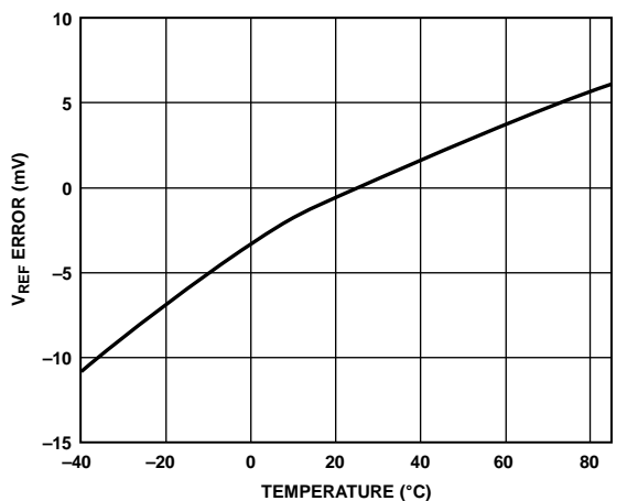
Figure 61. Typical V_{REF} = 1.3 V Drift
