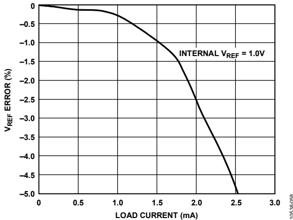
Figure 58. V_{REF} = 1.0V Error vs. Load Current
