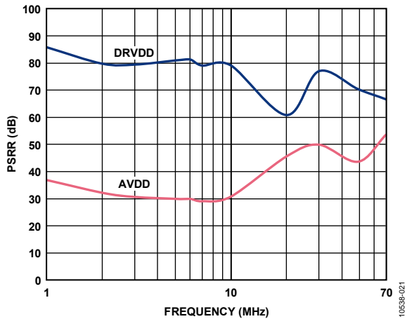
Figure 21. PSRR vs. Frequency, f_{SAMPLE} = 125 MSPS, V_{REF} = 1.0 V
