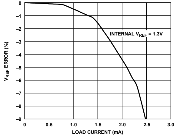
Figure 59. V_{REF} = 1.3V Error vs. Load Current
