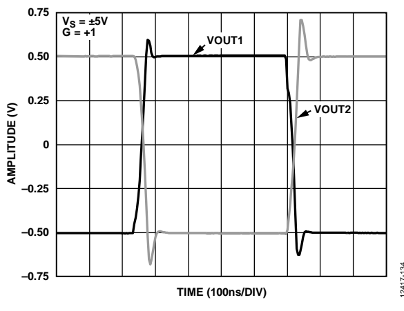
Figure 33. Large Signal Step Response (Single-Ended Output), V_S = \pm 5\text{ V}
