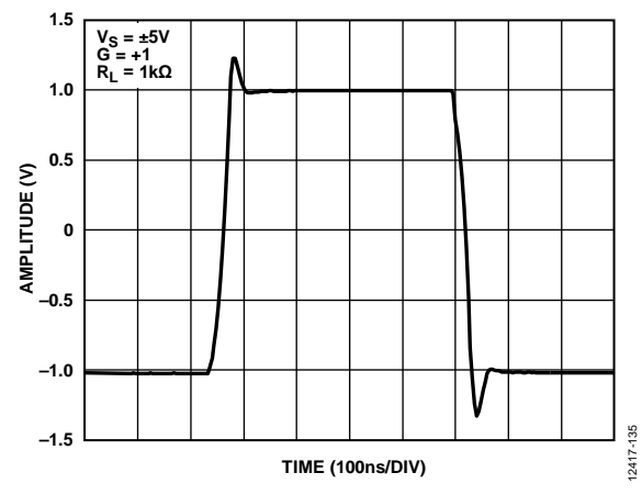
Figure 34. Large Signal Step Response (Differential Output), V_S = \pm 5\text{ V}
