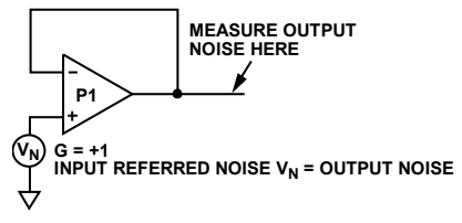
Figure 52. Input Referred Voltage Noise for P1
