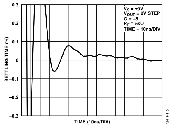
Figure 20. 0.1% Settling Time
