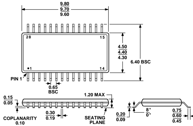
Figure 73. 28-Lead Thin Shrink Small Outline Package [TSSOP], (RU-28) Dimensions shown in millimeters
