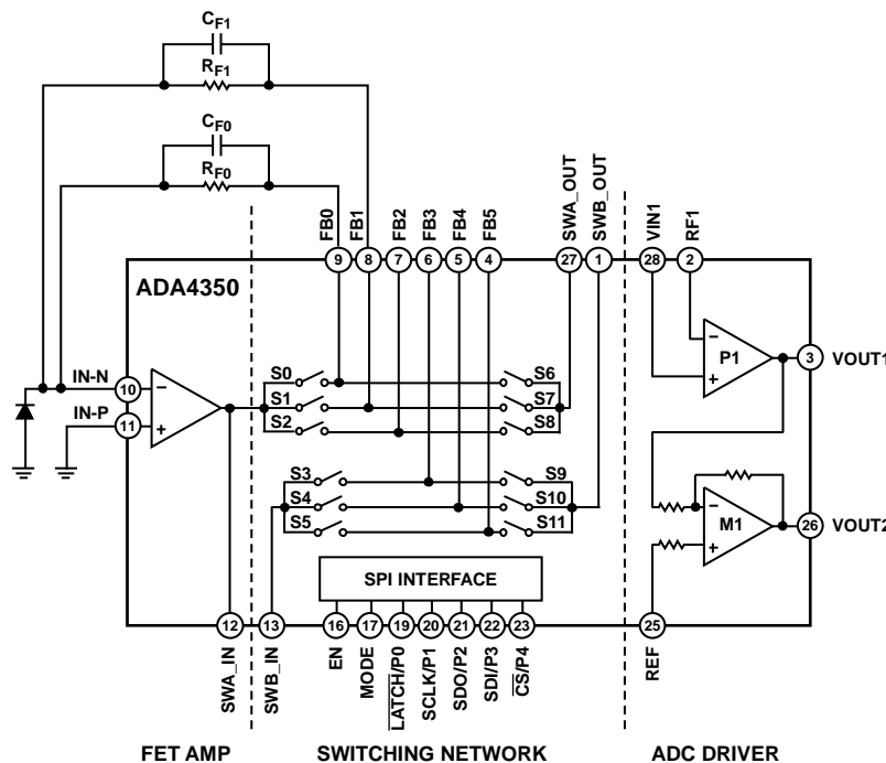
Figure 55. Simplified Schematic
