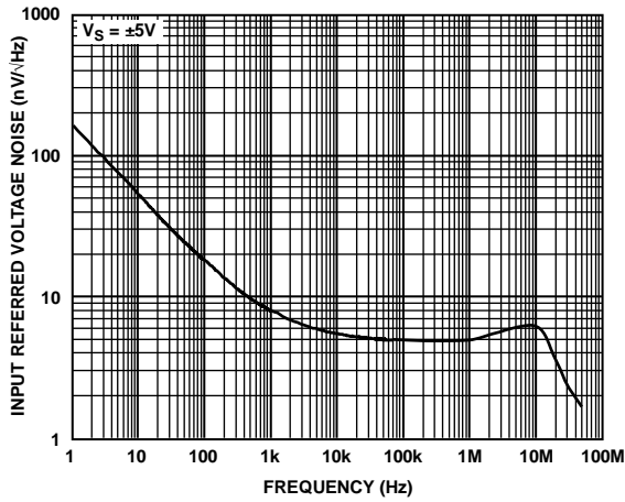
Figure 46. Input Referred Voltage Noise vs. Frequency, P1 Only, See Test Circuit Diagram in Figure 52
