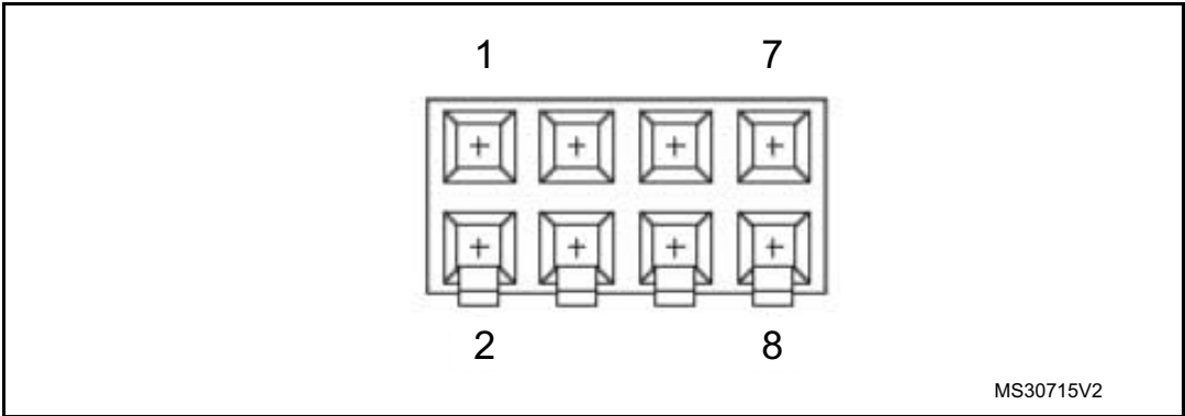
Figure 9. RF EEPROM daughter board connector CN2(Front View)
