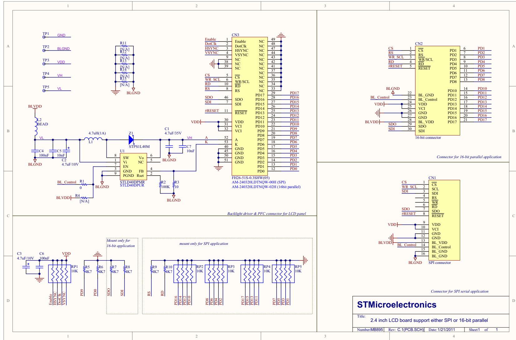
Figure 35. TFT LCD daughter board MB895
