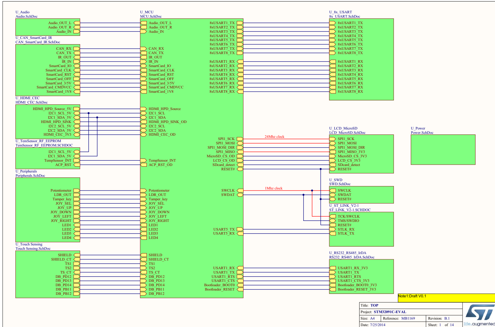
Figure 21. STM32091C-EVAL top view
