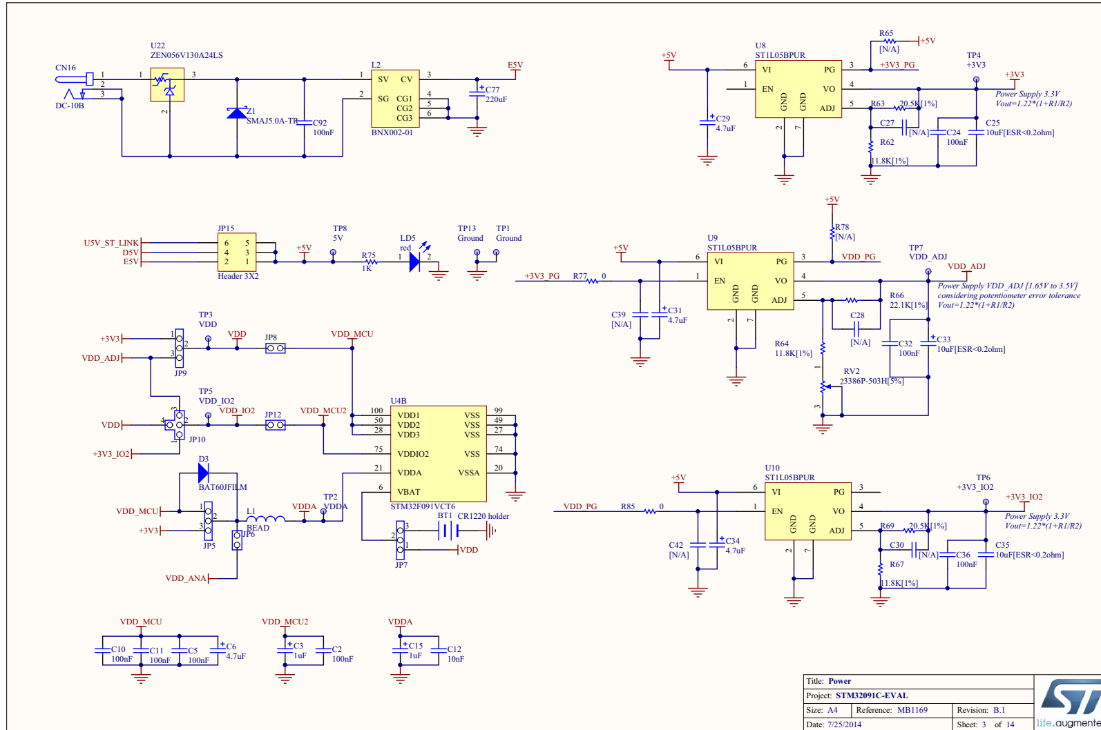
Figure 23. STM32091C-EVAL Power
