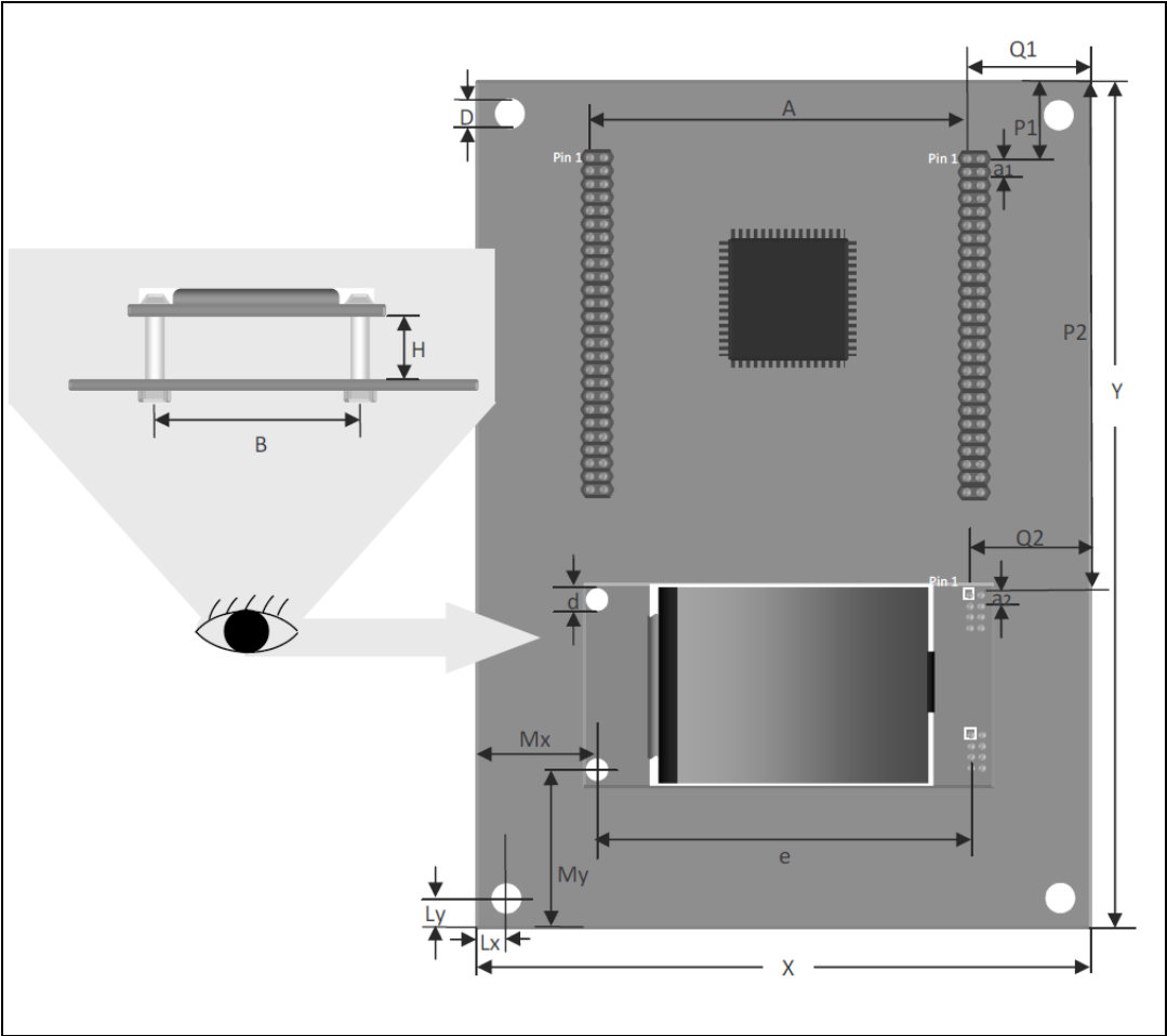
Figure 36. Mechanical dimensions
