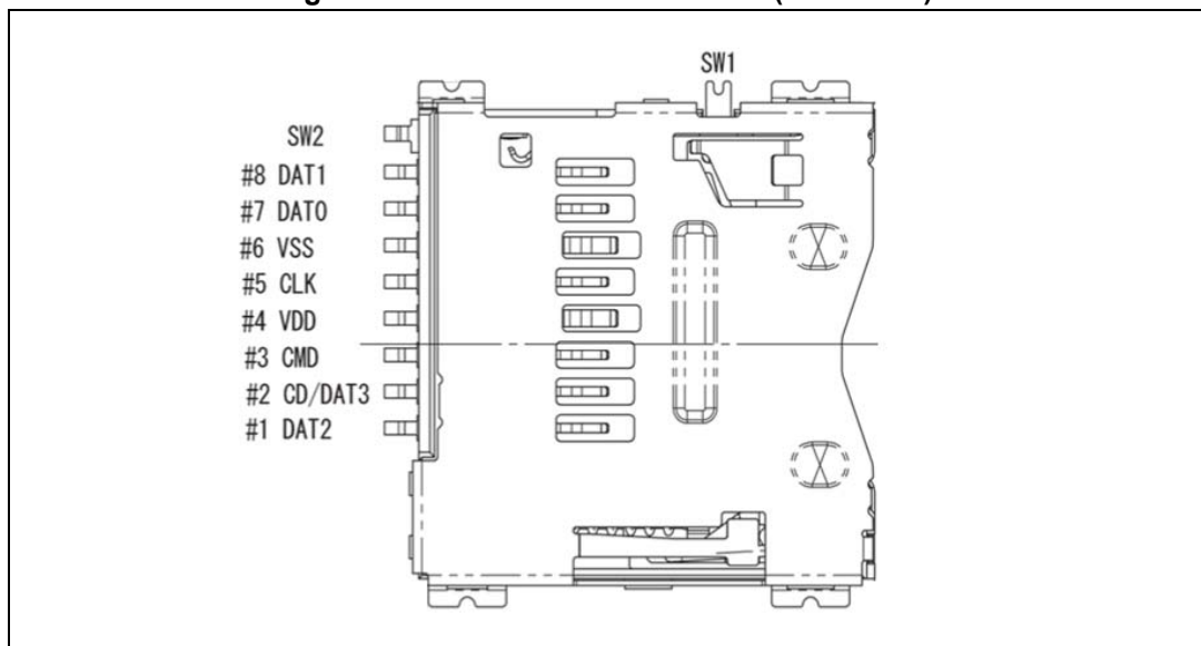
Figure 13. MicroSD connector CN8 (front view)
