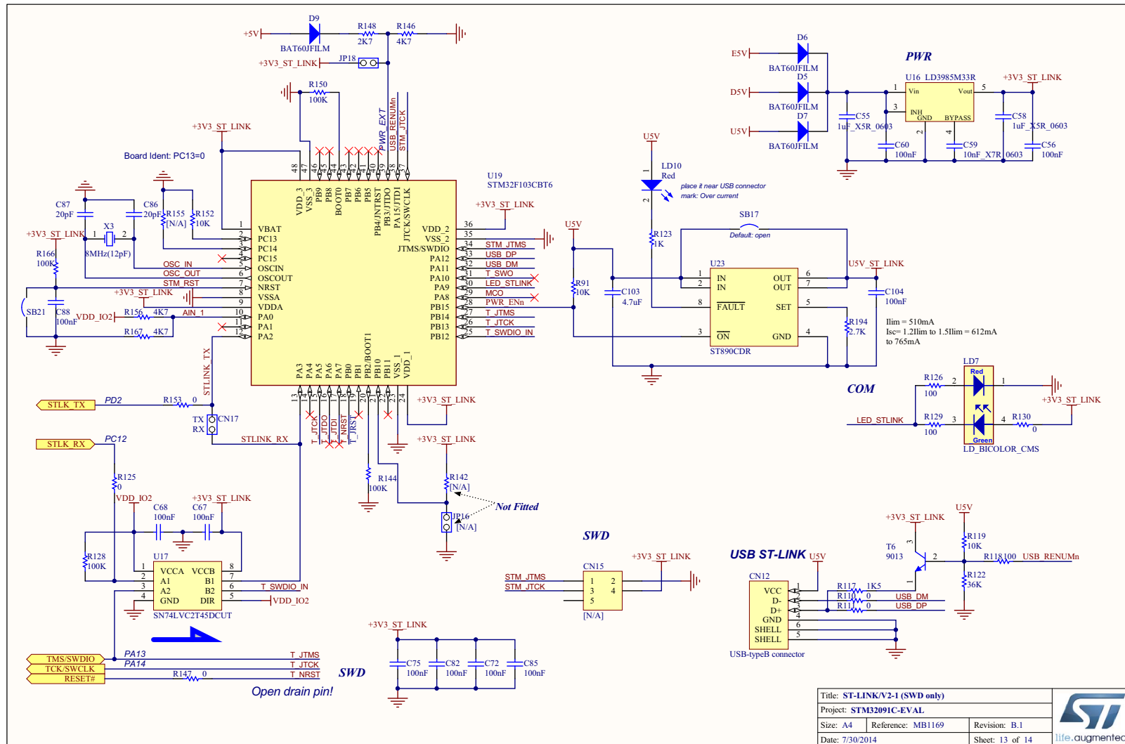
Figure 33. STM32091C-EVAL ST-LINK/V2-1 (SWD only)
