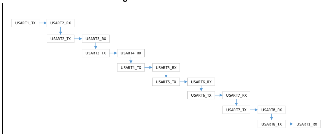
Figure 7. USART data flow
