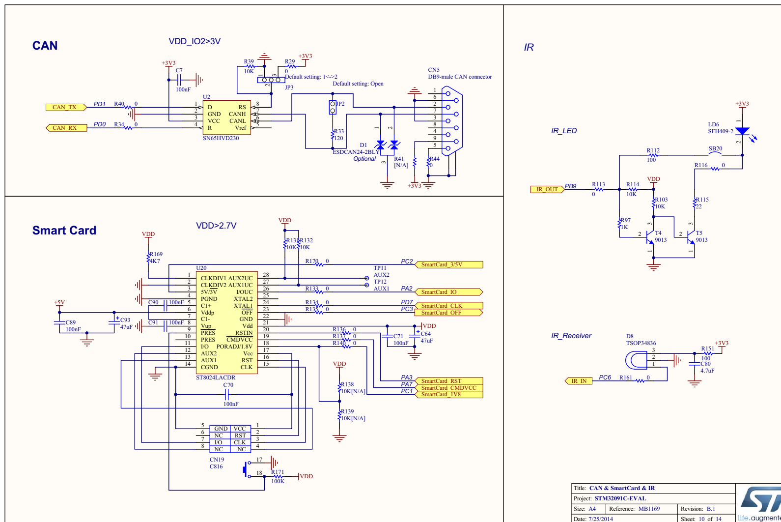
Figure 30. STM32091C-EVAL CAN, SmartCard and IR
