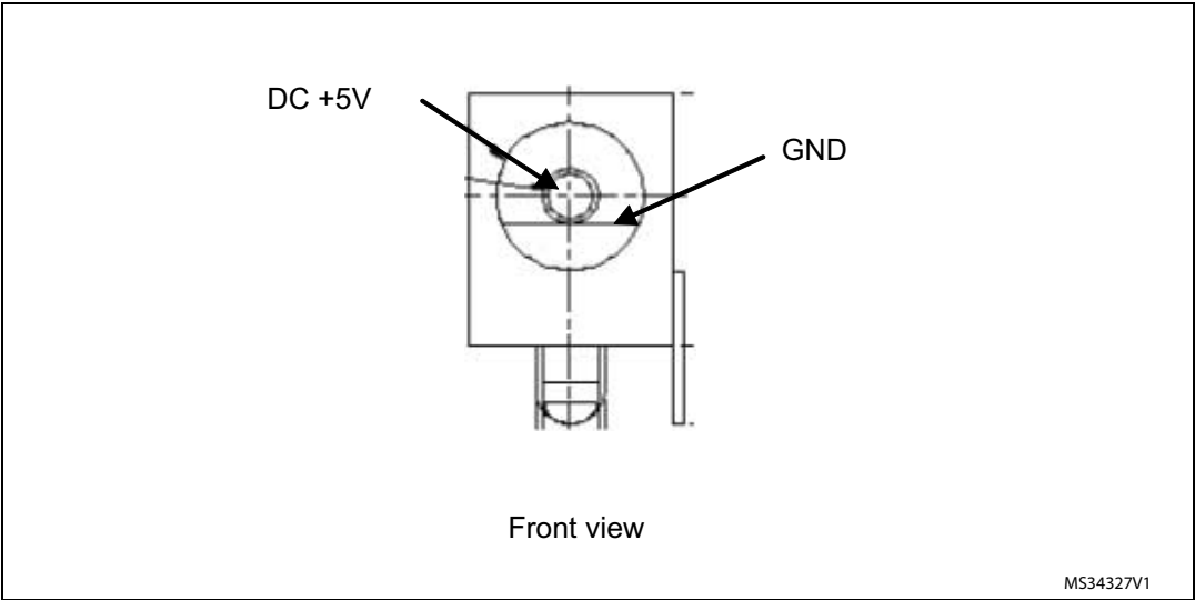
Figure 18. Power supply connector CN16
