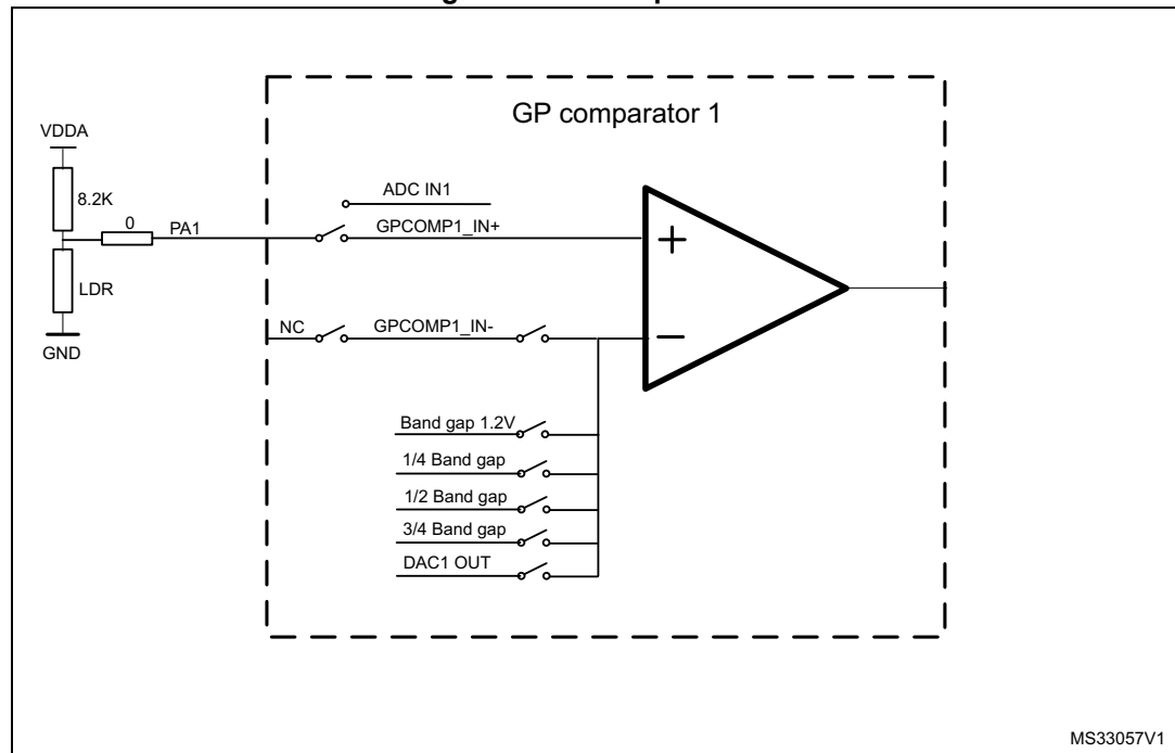
Figure 6. GP comparator 1
