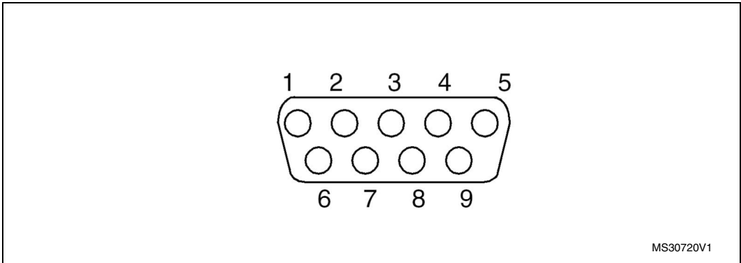
Figure 12. CAN D-type 9-pins male connector CN5 (front view)
