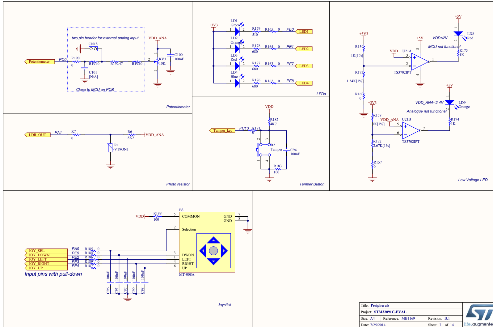
Figure 27. STM32091C-EVAL Peripherals
