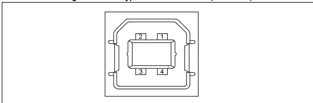
Figure 17. USB type B connector CN12 (front view)
