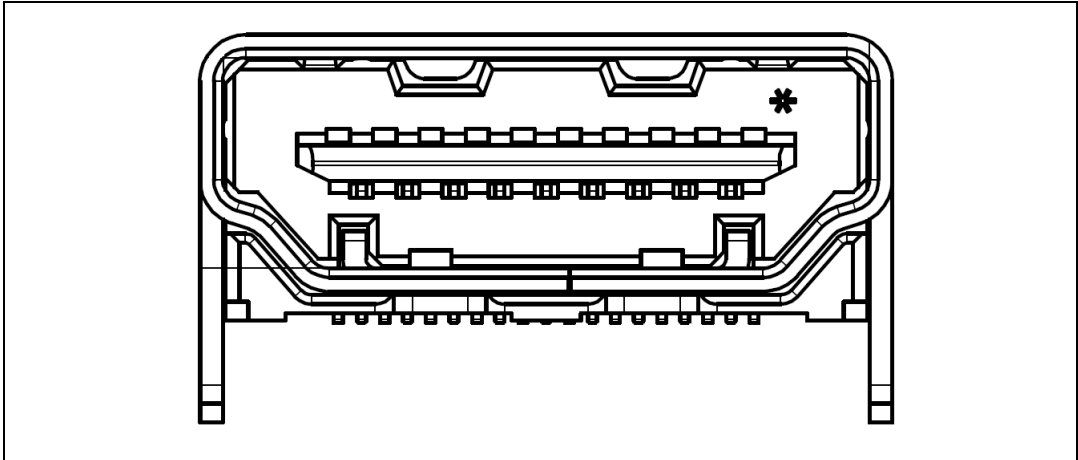
Figure 11. HDMI Source connectors CN4(front view)
