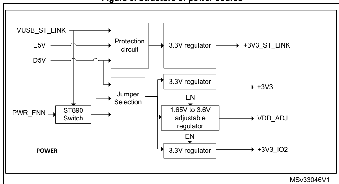
Figure 5. Structure of power source
