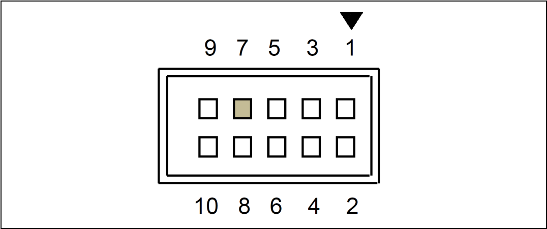
Figure 15. High density SWD debugging connector CN10 (top view)
