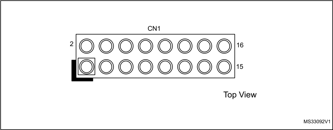
Figure 8. 8x USARTs connector CN1 Top View
