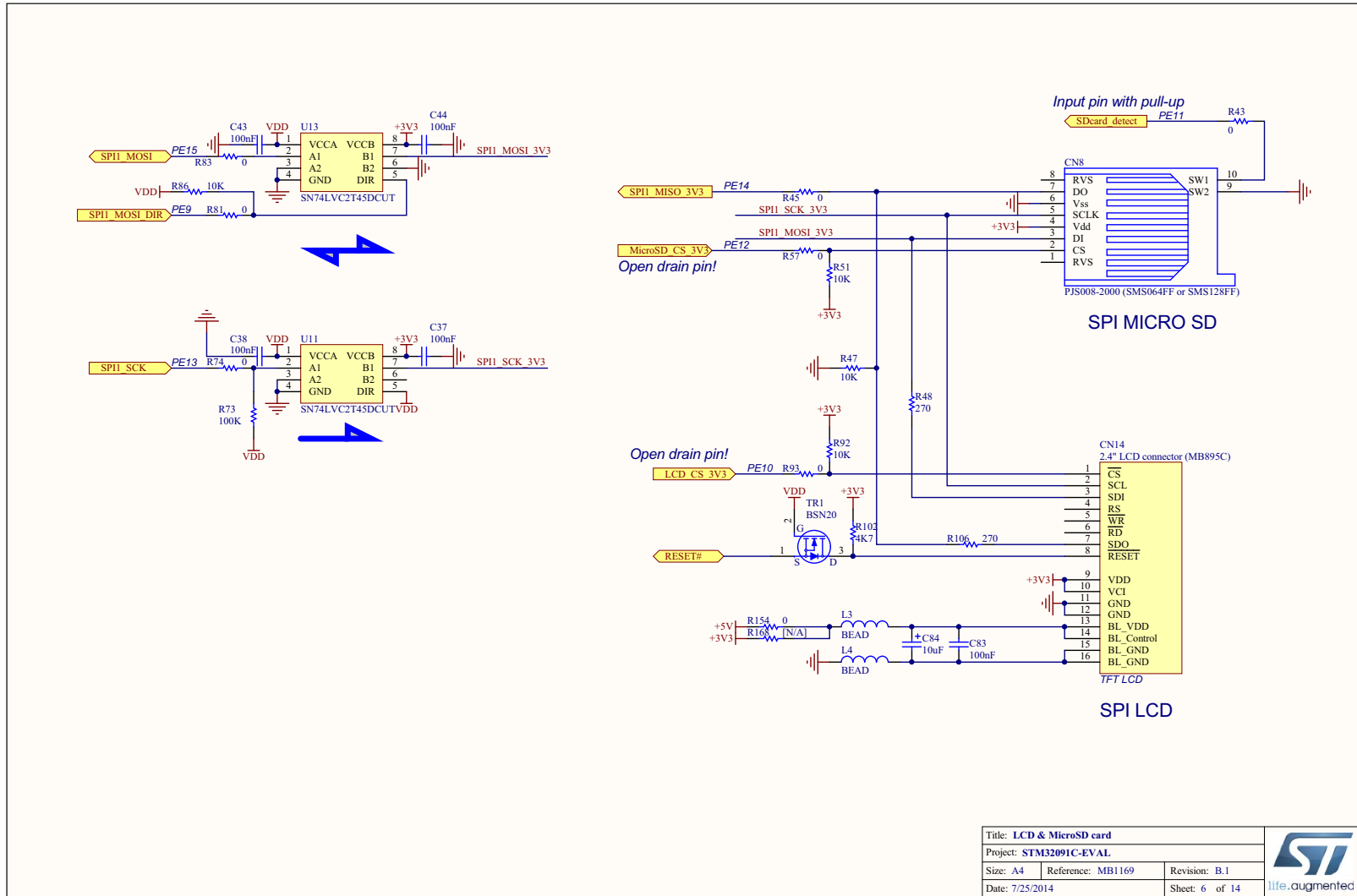
Figure 26. STM32091C-EVAL LCD and MicroSD card
