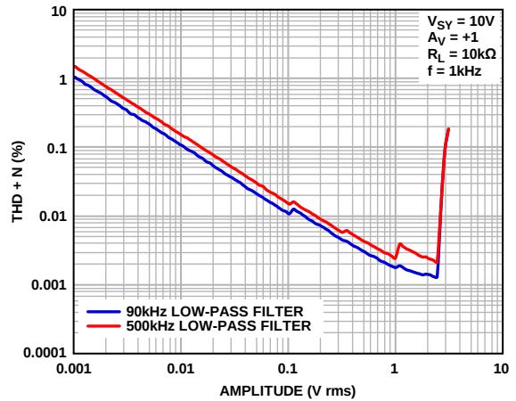
Figure 83. THD + N vs. Amplitude, V_{SV} = 10\text{ V}
