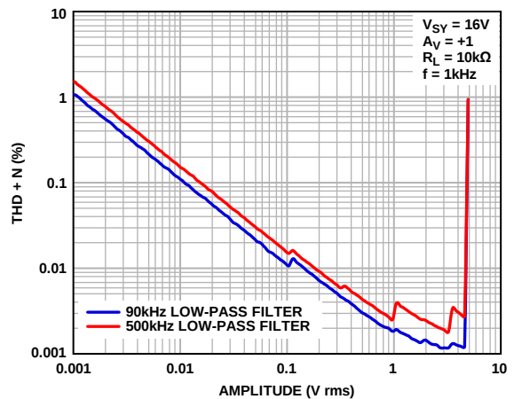
Figure 84. THD + N vs. Amplitude, V_{SV} = 16\text{ V}
