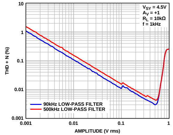
Figure 82. THD + N vs. Amplitude, V_{SV} = 4.5\text{ V}
