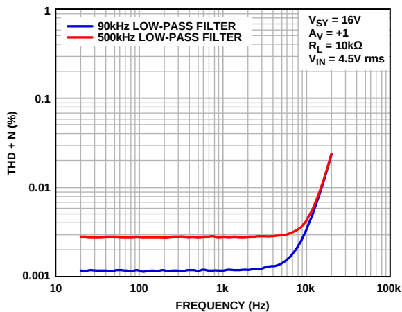
Figure 81. THD + N vs. Frequency, V_{SV} = 16\text{ V}
