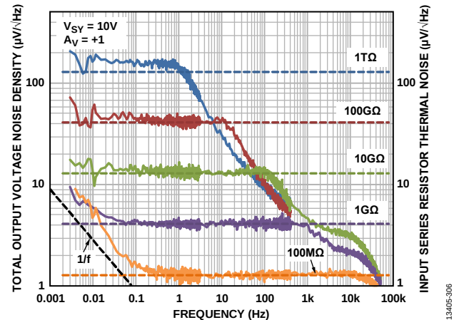
Figure 117. Transimpedance NSD Referred to Output
