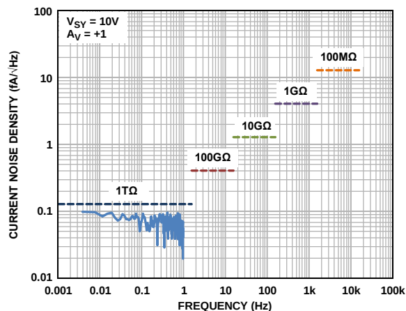
Figure 118. Current Noise Spectral Density
