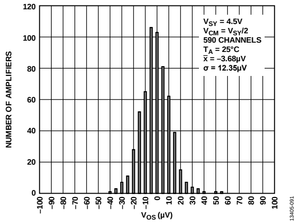
Figure 87. Input Offset Voltage Distribution, V_{SY} = 4.5\text{ V}
