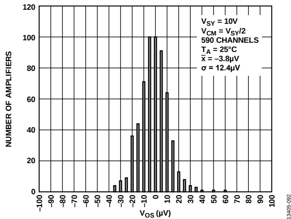
Figure 88. Input Offset Voltage Distribution, V_{SY} = 10\text{ V}
