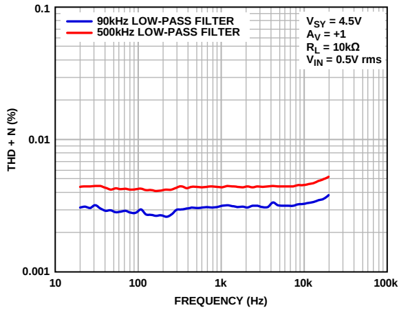
Figure 79. THD + N vs. Frequency, V_{SV} = 4.5\text{ V}
