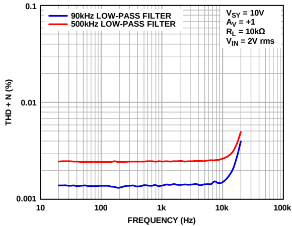
Figure 80. THD + N vs. Frequency, V_{SV} = 10\text{ V}
