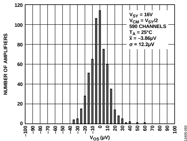
Figure 89. Input Offset Voltage Distribution, V_{SY} = 16\text{ V}
