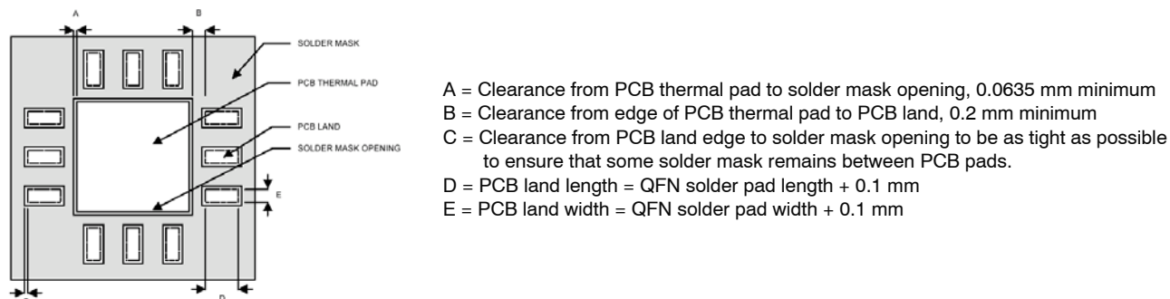
Figure 25. PCB Land and Solder Mask Recommendations
