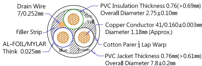
SJT 18AWGx3C Shielded(A+E) (Wire Cross-Section)
