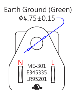
ME-301 (NEMA 5-15P) (Dimensions of Plug Face)
