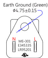
ME-301 (NEMA 5-15P) (Dimensions of Plug Face)
