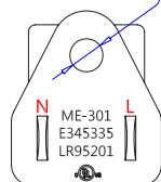
ME-301 (NEMA 5-15P) (Dimensions of Plug Face)
