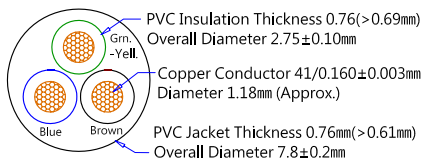
SJT 18AWGx3C (Wire Cross-Section)
