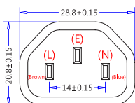
FM-7 (IEC 60320, C14) (Dimensions of Plug Face)
