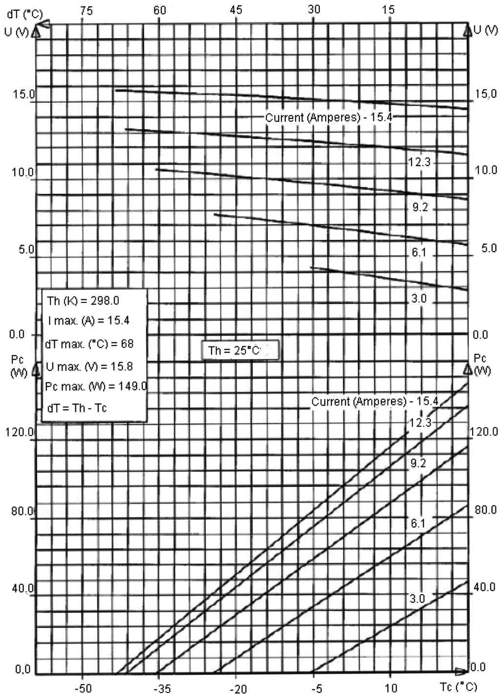
2-3 Performance Graph (298K)
