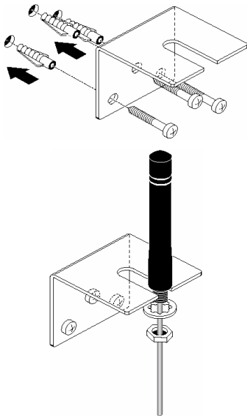
Figure 14 Wall mounting
