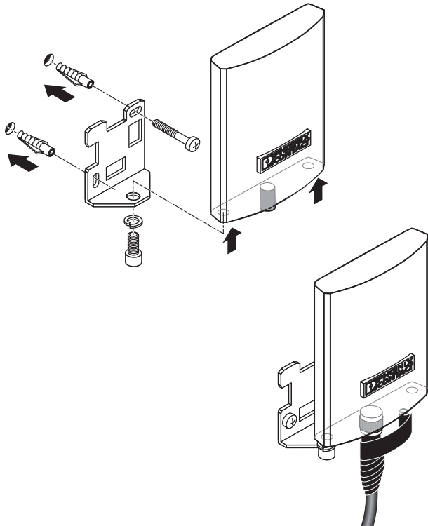
Figure 20 Wall mounting
