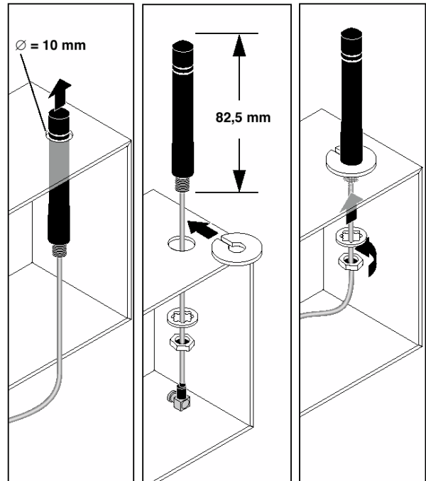
Figure 15 Hole mounting
