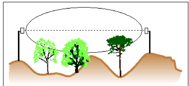
Figure 8 Fresnel zone adversely affected by obstacles
