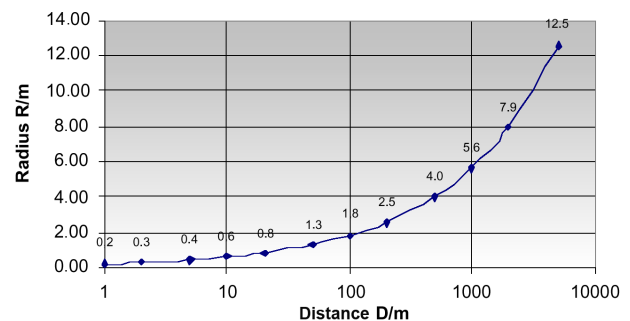
Figure 9 Radius R of the Fresnel zone over distance D
