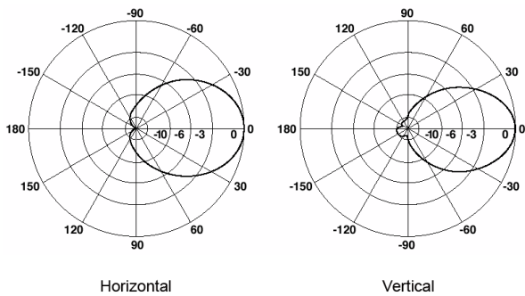
Figure 19 Directional characteristics
