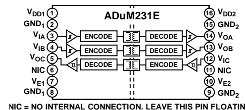
Figure 4. ADuM231E Functional Block Diagram
