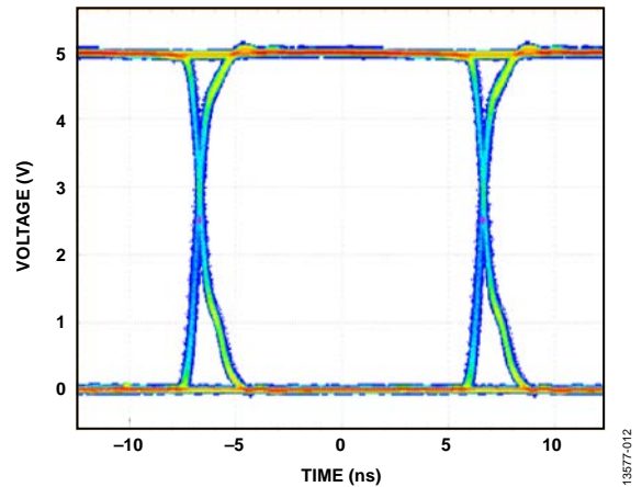
Figure 20. Eye Diagram
