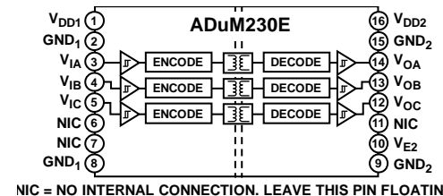
Figure 2. ADuM230E Functional Block Diagram
