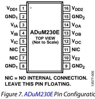
Figure 7. ADuM230E Pin Configuration
