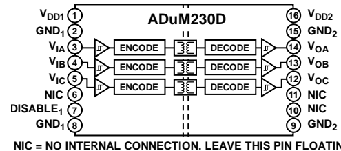
Figure 1. ADuM230D Functional Block Diagram
