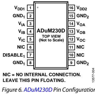
Figure 6. ADuM230D Pin Configuration
