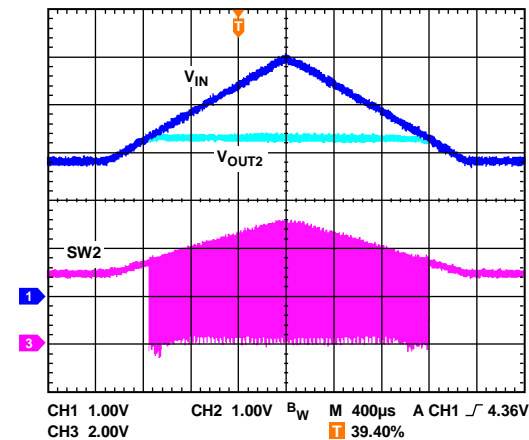
Figure 51. Channel 2 100% Duty Operation in PWM Mode
