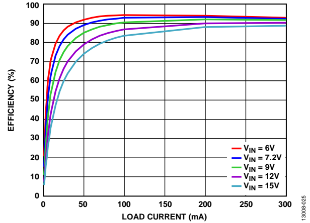
Figure 25. Channel 2 PWM Efficiency vs. Load Current, V_{OUT2} = 5\text{ V}
