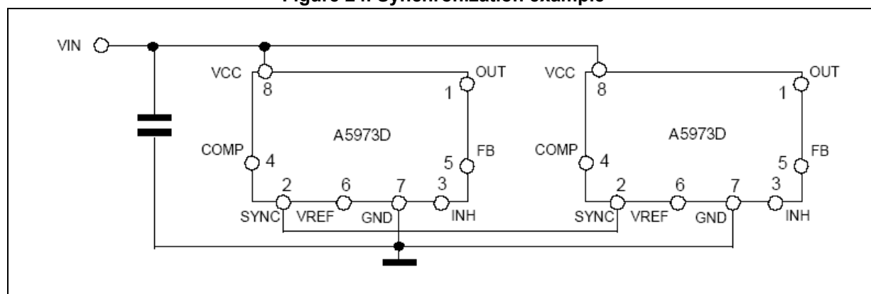
Figure 24. Synchronization example
