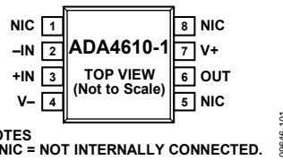
Figure 2. ADA4610-1 Pin Configuration, 8-Lead SOIC (R Suffix)
