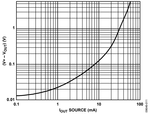
Figure 21. Dropout Voltage ( V+ - V_{out} ) vs. I_{out Source} , V_{SY} = \pm 5 V
