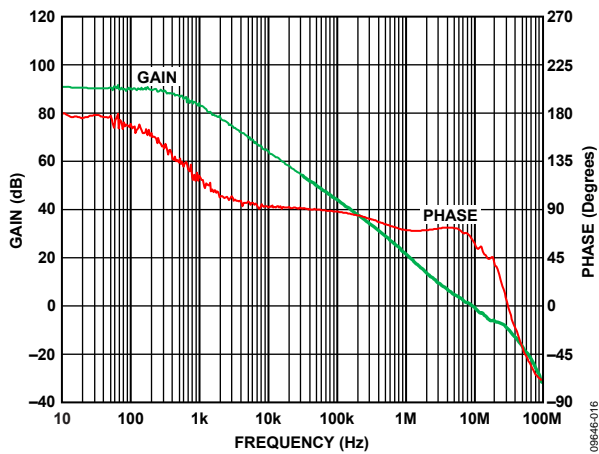
Figure 23. Open-Loop Gain and Phase vs. Frequency, V_{SY} = \pm 5 V , R_L = 2 k\Omega , V_{IN} = 5 mV
