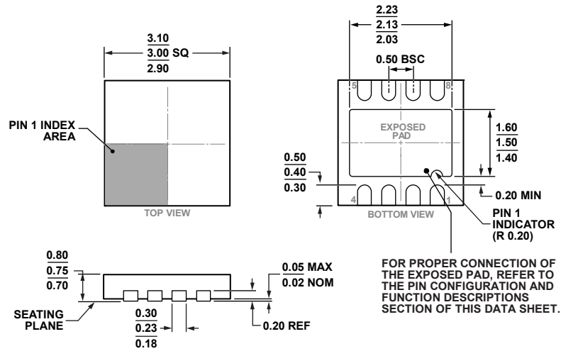
Figure 64. 8-Lead Lead Frame Chip Scale Package [LFCSP] 3 mm x 3 mm Body and 0.75 mm Package Height (CP-8-20)
