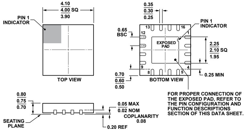
Figure 66. 16-Lead Lead Frame Chip Scale Package [LFCSPP] 4 mm x 4 mm Body and 0.75 mm Package Height (CP-16-23)
