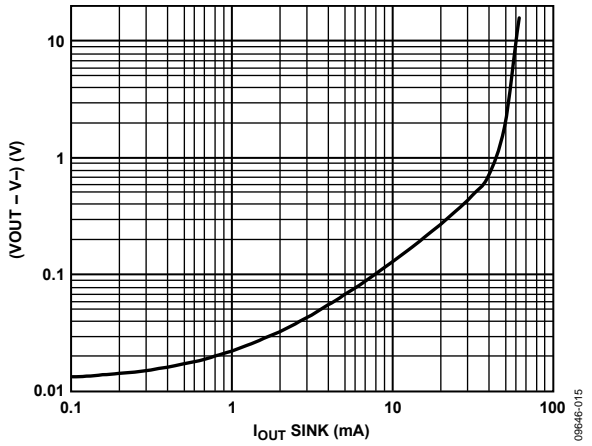
Figure 22. Dropout Voltage ( V_{out} - V- ) vs. I_{out Sink} , V_{SY} = \pm 5 V
