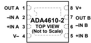
Figure 6. ADA4610-2 Pin Configuration, 8-Lead LFCSP (CP Suffix)
