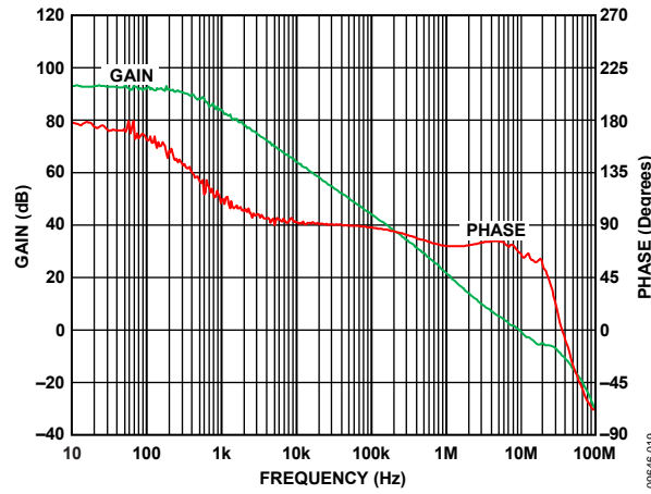
Figure 26. Open-Loop Gain and Phase vs. Frequency, V_{SY} = \pm 15 V , R_L = 2 k\Omega , V_{IN} = 5 mV
