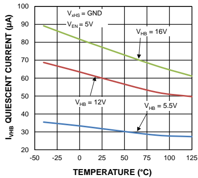
V HB Quiescent Current (All Channels) vs. Temperature
