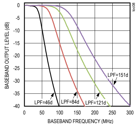
BASEBAND FILTER FREQUENCY RESPONSE
