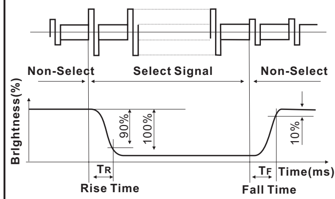
DEFINITION OF OPTICAL RESPONSE TIME T_R & T_F
