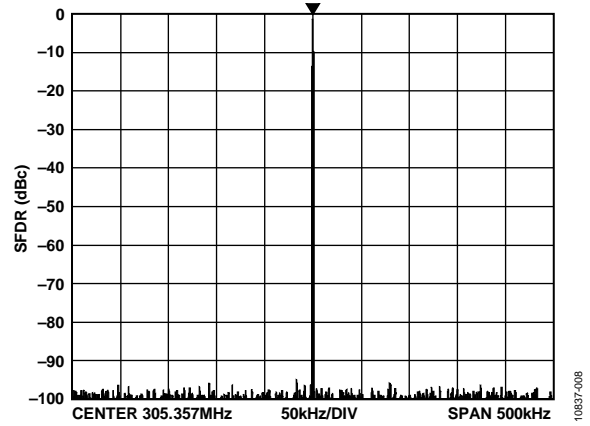
Figure 8. Narrow-Band SFDR at 305.3 MHz, SYSCLK = 2.5 GHz (SYSCLK PLL Bypassed)
