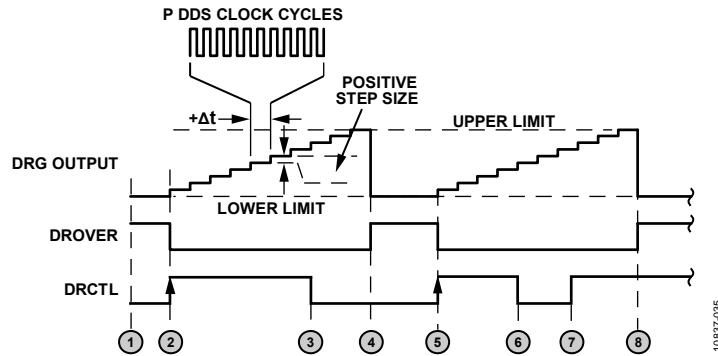
Figure 39. No-Dwell High Ramp Generation
