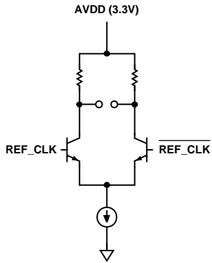
Figure 27. REF CLK input
