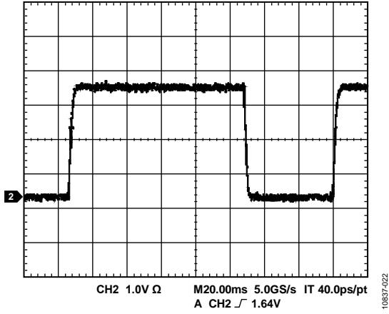
Figure 22. SYNC_OUT ( f_{\text{SYSCLK}}/384 )
