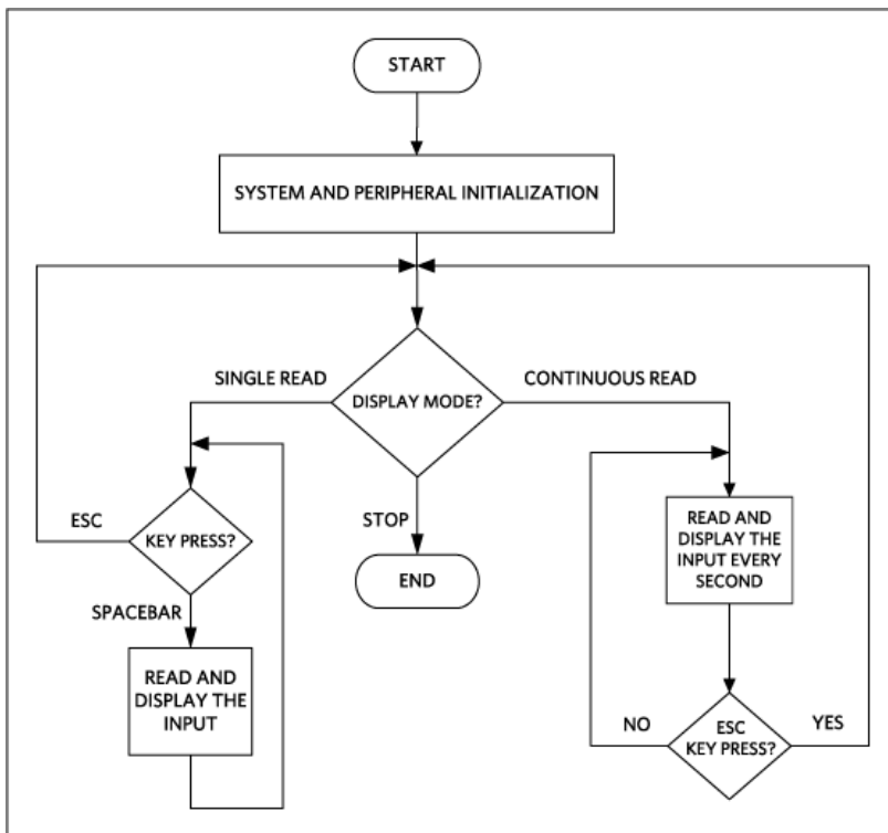
Figure 2. The MAXREFDES64# firmware flowchart.
