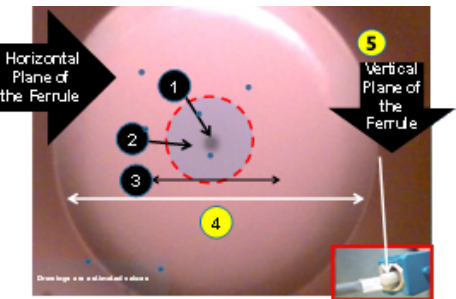
Figure 5 – Zones of end face
