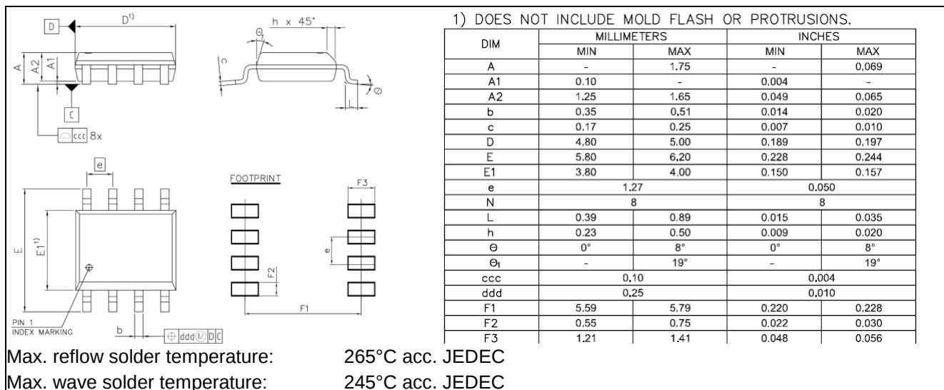
Figure 12 Package drawing
