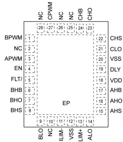
MIC4607-2 28-Pin 4mm × 5mm (ML) (Top View)
