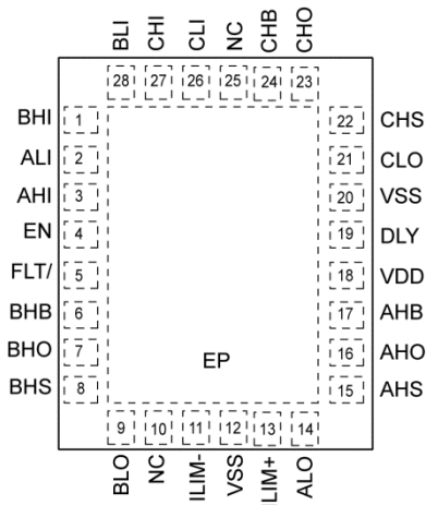
MIC4607-1 28-Pin 4mm × 5mm (ML) (Top View)
