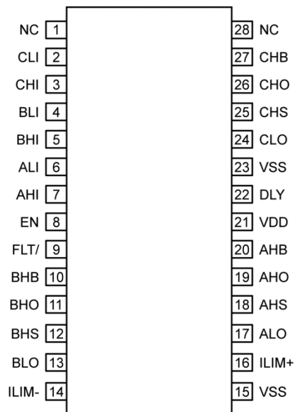
MIC4607-1 28-Pin TSSOP (TS) (Top View)
