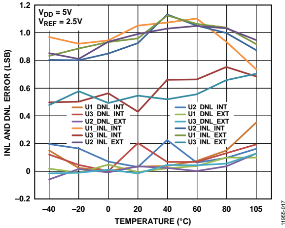
Figure 17. INL and DNL Error vs. Temperature (AD5683R/AD5683)
