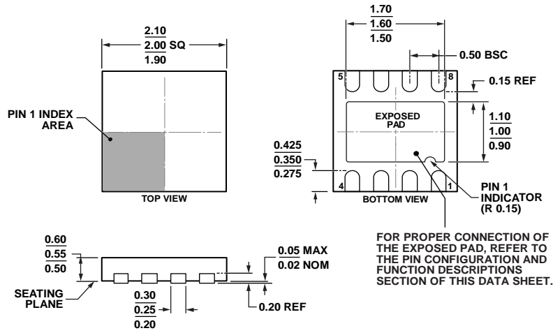
Figure 56. 8-Lead Lead Frame Chip Scale Package [LFCSF_UD] 2.00 mm × 2.00 mm Body, Ultra Thin, Dual Lead (CP-8-10) Dimensions shown in millimeters
