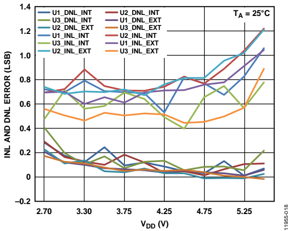
Figure 18. INL and DNL Error vs. Supply Voltage
