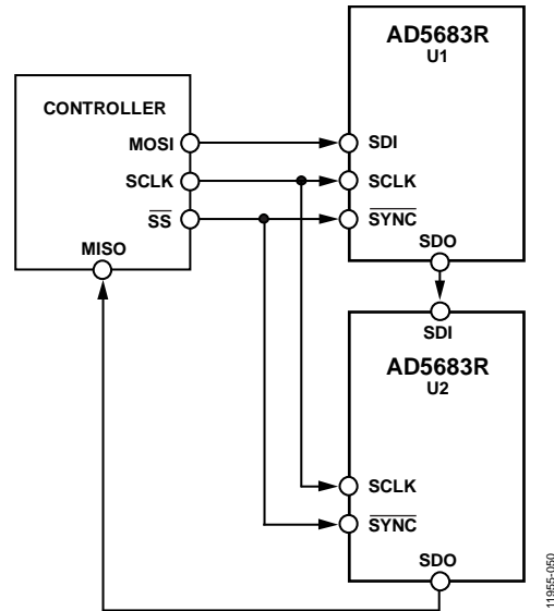
Figure 50. Daisy-Chain Connection
