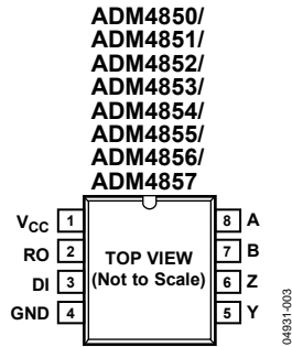
Figure 5. 8-Lead SOIC Pin Configuration, ADM4850/ADM4851/ADM4852/ADM4853/ADM4854/ADM4855/ADM4856/ADM4857
