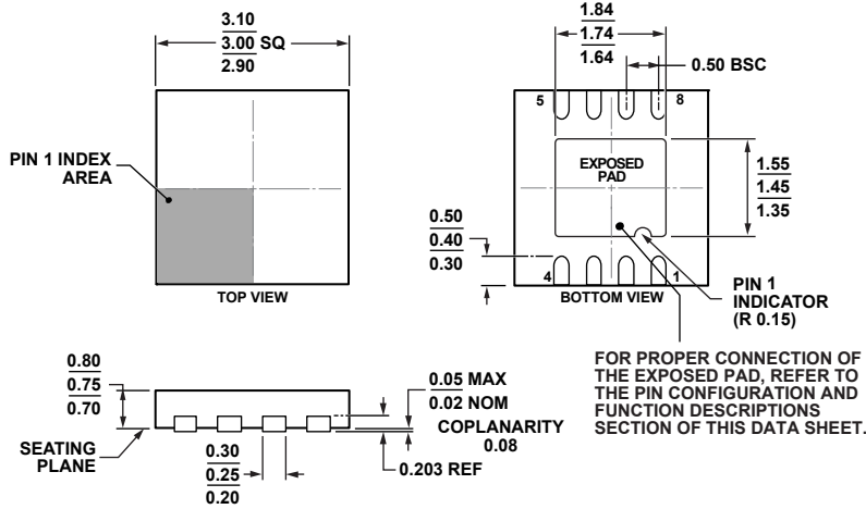
Figure 32. 8-Lead Lead Frame Chip Scale Package [LFCSP] 3 mm x 3 mm Body and 0.75 mm Package Height (CP-8-13) Dimensions shown in millimeters
