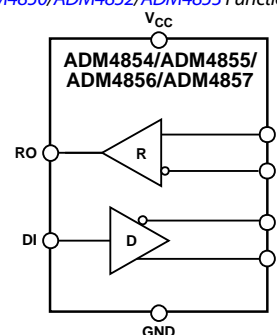
Figure 2. ADM4854/ADM4855/ADM4856/ADM4857 Functional Block Diagram
