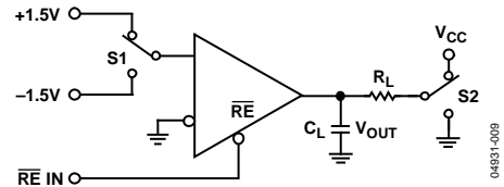
Figure 23. Receiver Enable/Disable (ADM4850/ADM4852/ADM4853)
