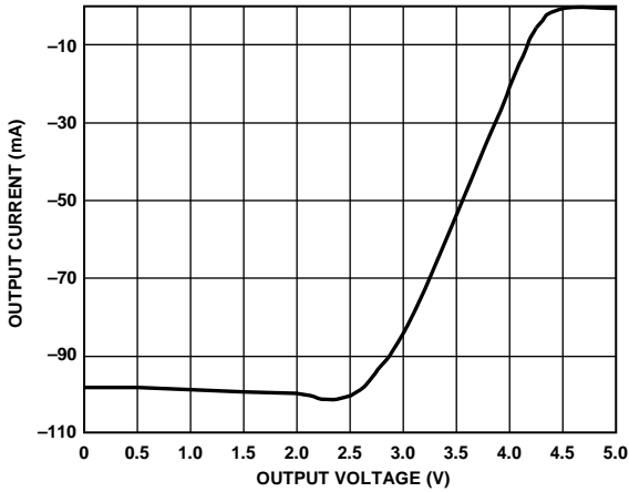
Figure 13. Output Current vs. Driver Output High Voltage
