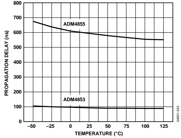
Figure 15. Receiver Propagation Delay vs. Temperature (ADM4853/ADM4855)
