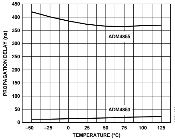
Figure 14. Driver Propagation Delay vs. Temperature (ADM4853/ADM4855)
