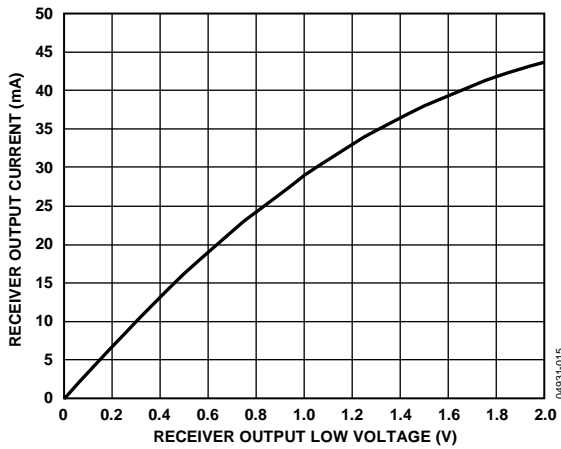
Figure 7. Receiver Output Current vs. Receiver Output Low Voltage
