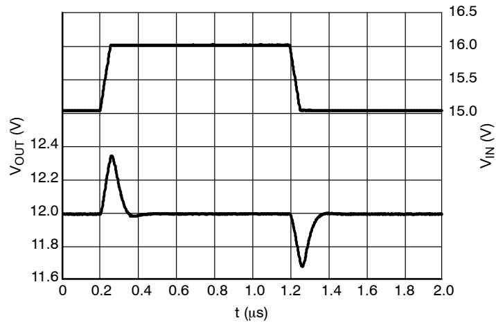
Figure 29. Line Transients, 12.0 V Version, t_R = t_F = 50 \mu\text{s} , I_{OUT} = 1 \text{ mA}
