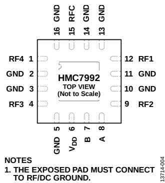
Figure 4. Pin Configuration
