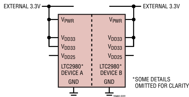
Figure 2. Powering LTC2980 from External 3.3V Supply
