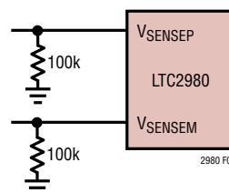
Figure 3. Undedicated Pull-Up Resistors
