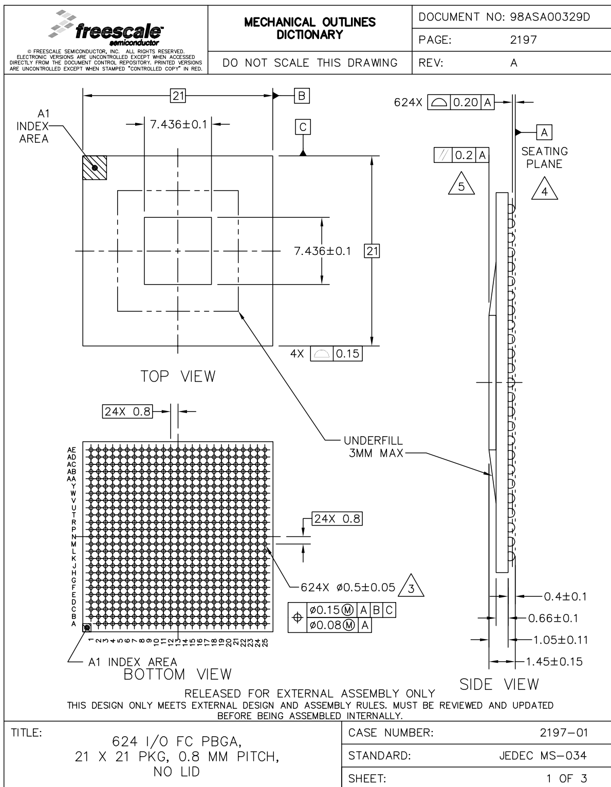
Figure 106. 21 x 21 mm Bare Die Package Top, Bottom, and Side Views (Sheet 1 of 2)
