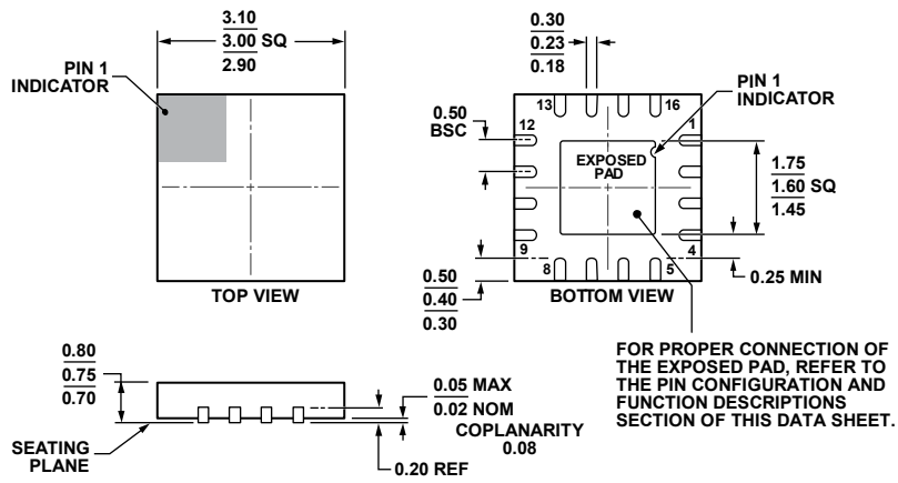
Figure 27. 16-Lead Lead Frame Chip Scale Package [LFCSP] 3 mm × 3 mm Body and 0.75 mm Package Height (CP-16-22)
