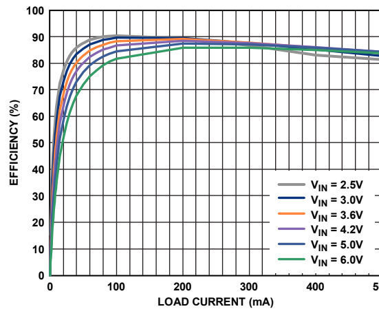
Figure 9. PWM Efficiency vs. Load Current, V_{OUT} = 1.2\text{ V}
