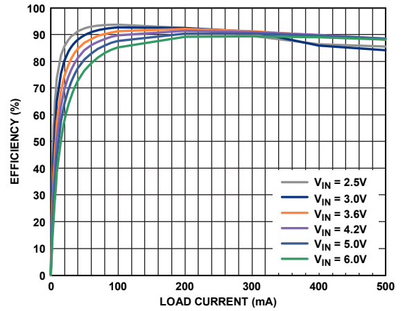
Figure 13. PWM Efficiency vs. Load Current, V_{OUT} = 1.8V
