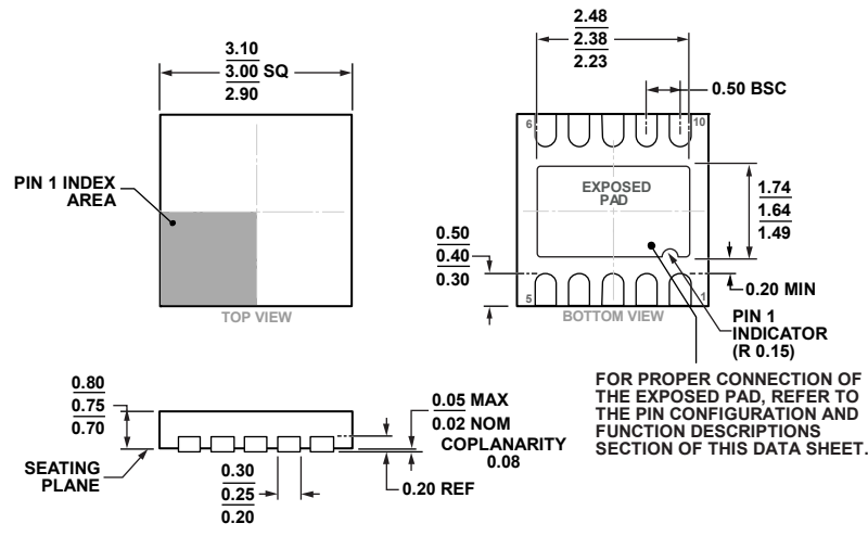
Figure 45. 10-Lead Lead Frame Chip Scale Package [LFCS] 3 mm × 3 mm Body and 0.75 mm Package Height (CP-10-9) Dimensions shown in millimeters
