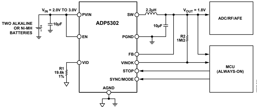
Figure 44. Typical Application Circuit with 2 Alkaline or NiMH Batteries
