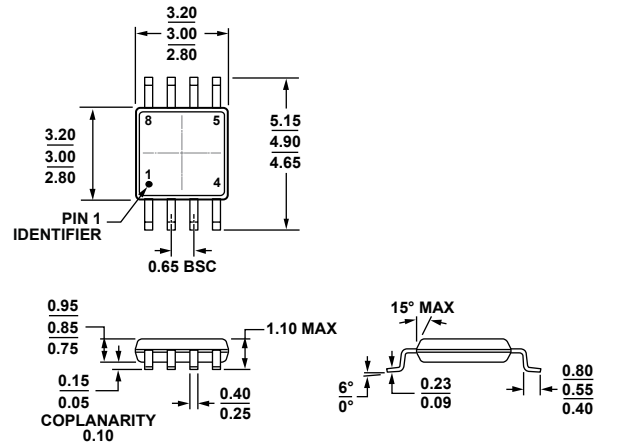
Figure 54. 8-Lead Mini Small Outline Package [MSOP] (RM-8)
