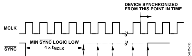
Figure 46. Recommended \overline{\text{SYNC}} Timing
