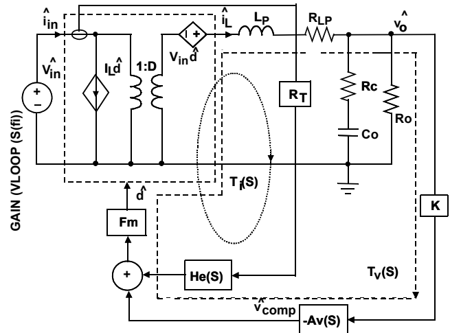
FIGURE 56. SMALL SIGNAL MODEL OF SYNCHRONOUS BUCK REGULATOR
