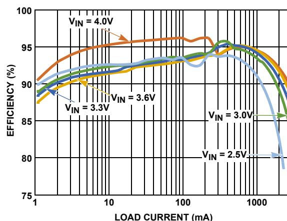
FIGURE 2. EFFICIENCY: V_{OUT} = 3.3V , T_A = +25^\circ C
