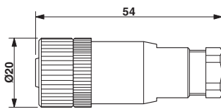
Dimensional drawing
