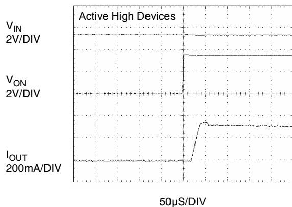
Figure 21. Current Limit Response Time (Output Shorted to GND by 10 \Omega , moderate short)
