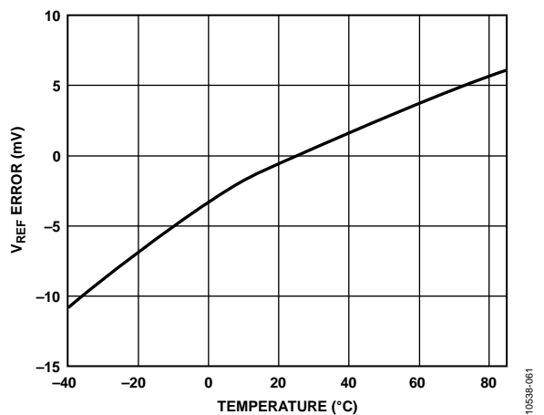
Figure 61. Typical V_{REF} = 1.3 V Drift
