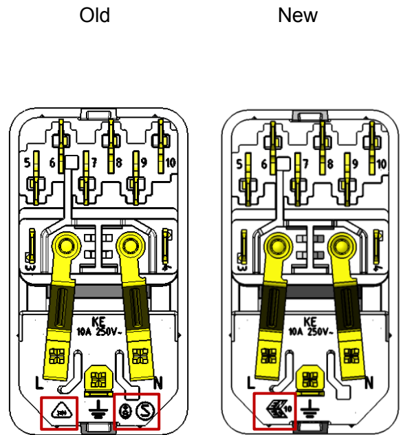
Snap-in version; Rear view
