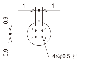
Size 7, 4 conductors
