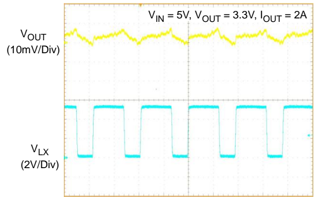
Time (500ns/Div)
