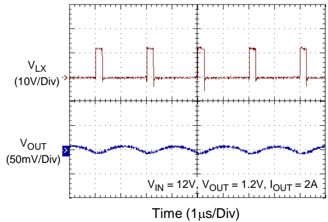
Voltage Ripple
