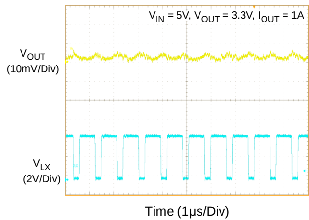
Voltage Ripple
